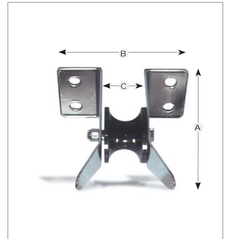
BOW ROLLER Anchors 15 kg/33 lbs.-30 kg/66 lbs.
