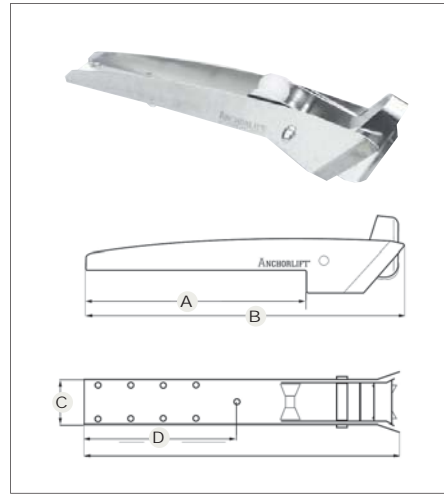
BOW ROLLER Anchor 8 kg/17 lbs.-20 kg/44 lbs.
