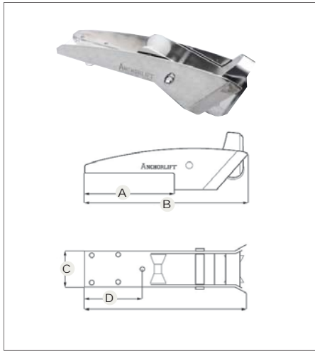
BOW ROLLER Anchors 8 kg/17 lbs.-15 kg/33 lbs.
