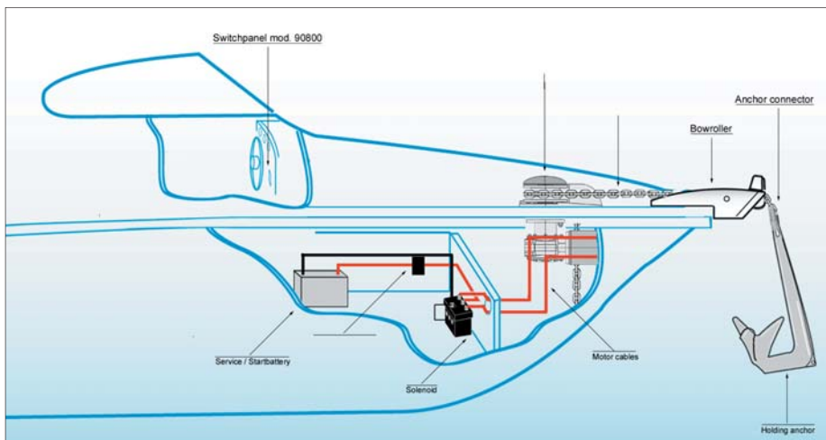
Motorboat installation vertical windlass, flush model with 2 wire motor.
