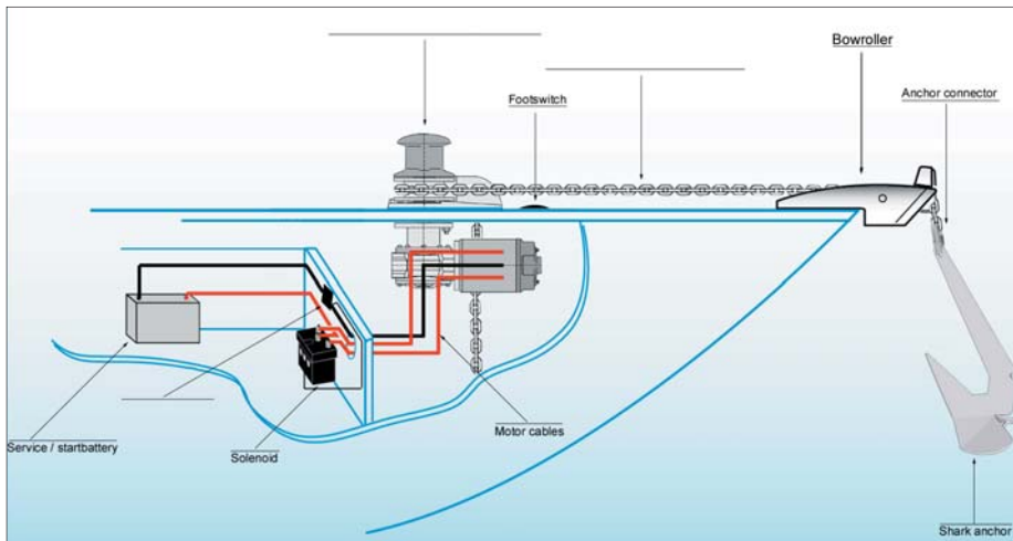
Sailboat installation vertical windlass, capstan model with 3 wire motor
